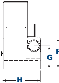
VS-550, 1200 and 1500 Dust Drawer
